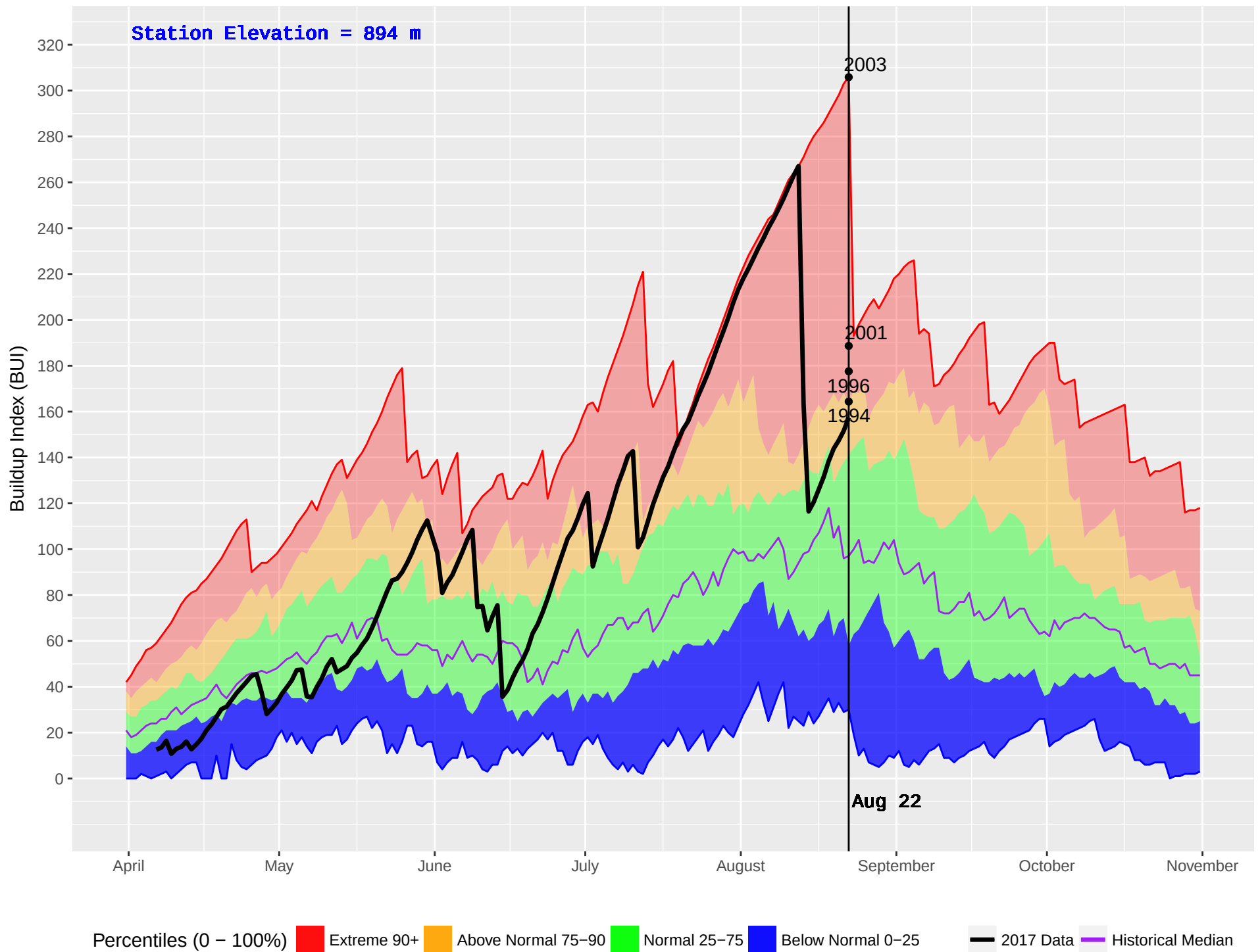
TOBY HUB (417) : Historical (1986–2016) and Current (2017) Noon Buildup Index (BUI)
