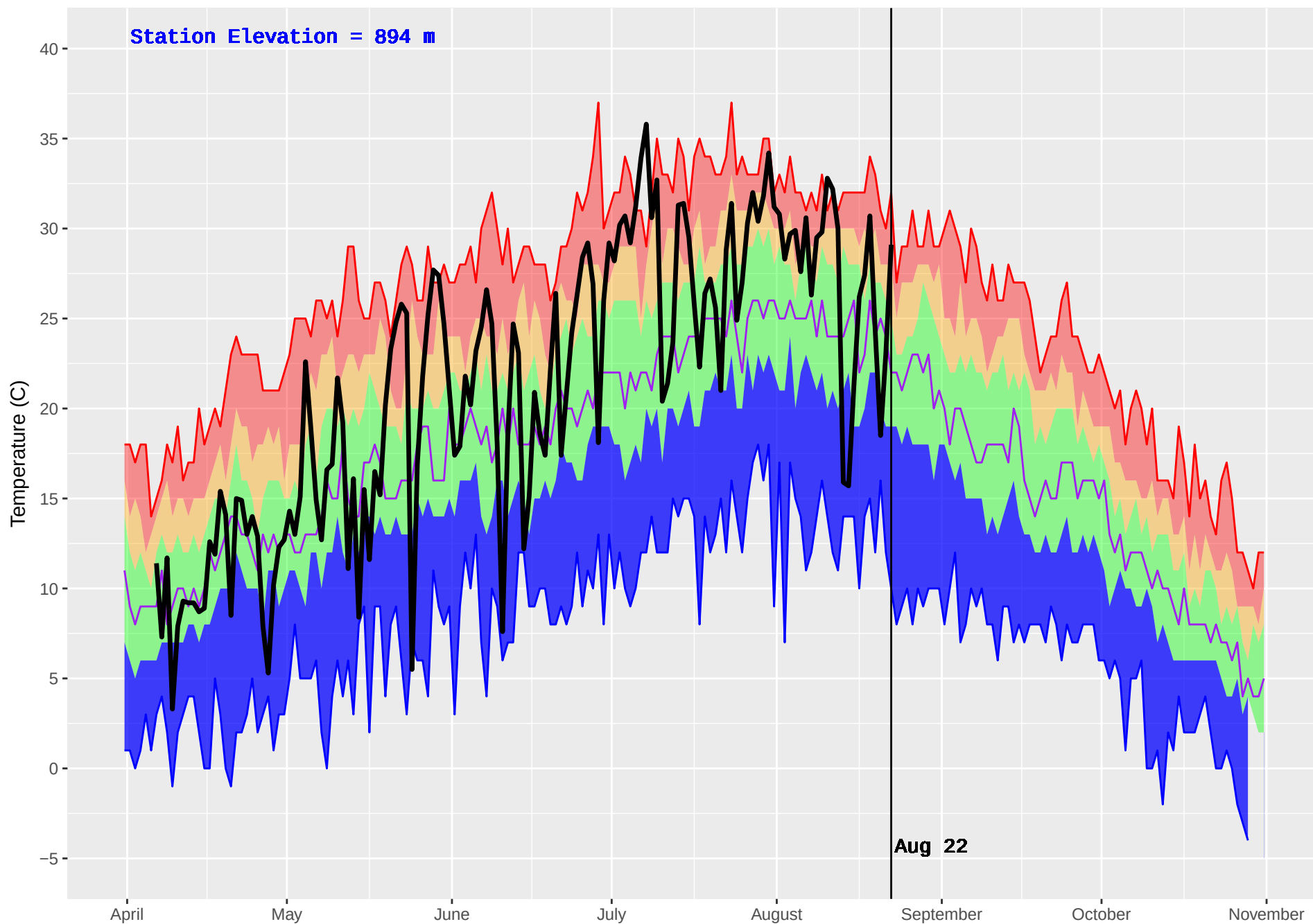
TOBY HUB (417) : Historical (1986–2016) and Current (2017) Noon Temperature
