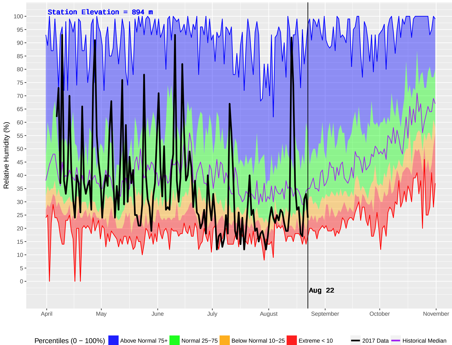
TOBY HUB (417) : Historical (1986–2016) and Current (2017) Noon Relative Humidity
