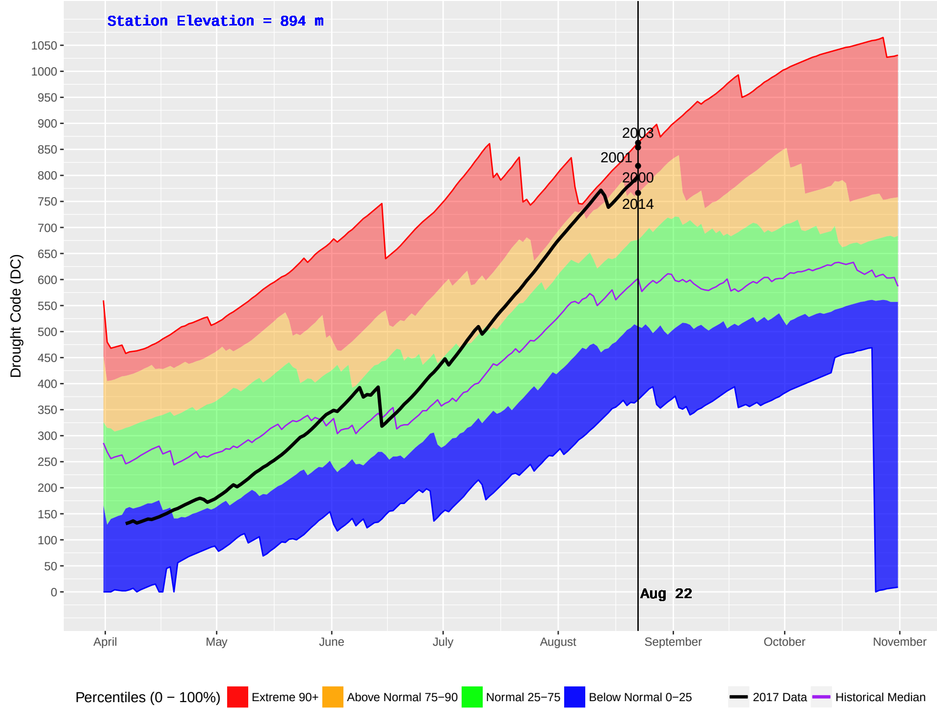
TOBY HUB (417) : Historical (1986–2016) and Current (2017) Noon Drought Code (DC)
